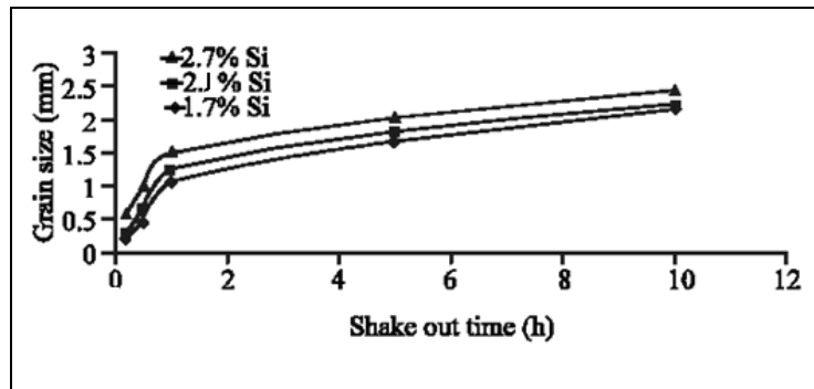
Fig.2: Plot of effect of shake-out time on grain size
