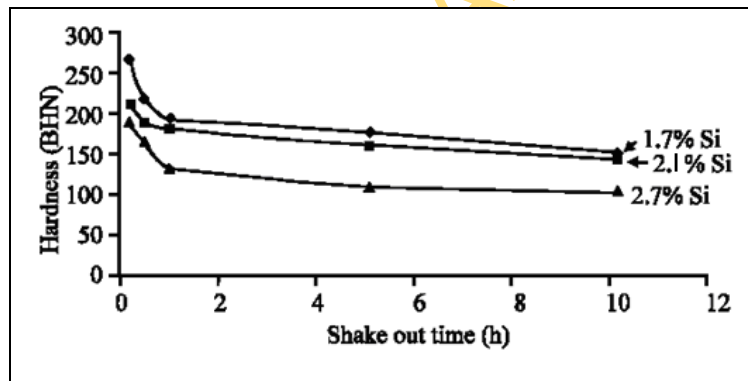
Fig.3: Plot of effect of shake-out time on hardness
