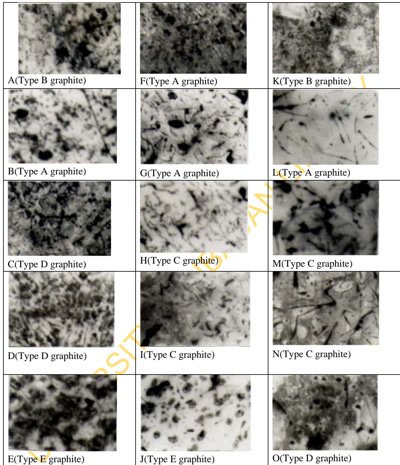
Fig.1: Optical micrographs of GL 250 cast in sand mould. Pouring Temperature-1400 0 C X100 A-E-Cast Iron containing 1.7% Si. (A=12mins,B=30mins,C=1hr,D=5hrs,E=10hrs) F-J-Cast iron containing 2.1% Si (F=12,G=30mins,H=1hr,I=5hrs,J=10hrs) K-O -Cast iron containing 2.7% Si (K=12,L=30mins,M=1hr,N=5hrs,O=10hrs)
